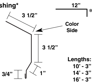
Shingle Rake Trim (P-SRT)
