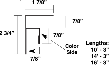
F and J x 7/8" (P-FJ-7/8)
