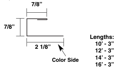
F and J x 7/8" (P-FJ-7/8)
