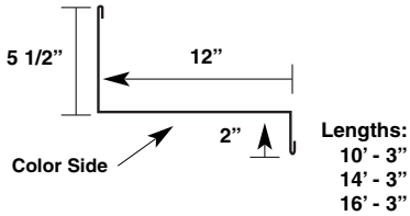
Eave Flashing* (P-EF)*
