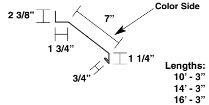
Soffit Flashing x 3 (P-SF3)
