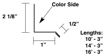
Rodent Guard (P-RG-71)
