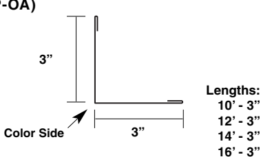
Outside Angle (P-OA)
