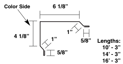
High Side Trim* (P-HST)*
