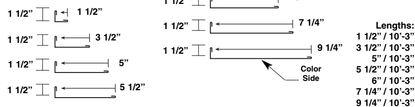
Wide J (P-WJ)
