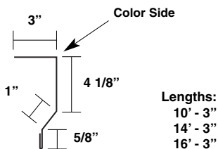
High Side Tie-In* (P-SWF)
